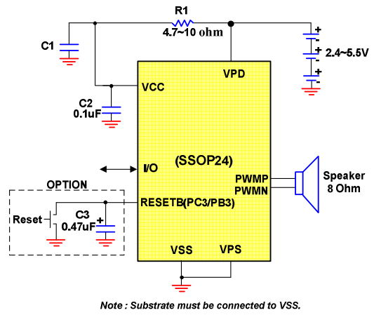
Figure 14. PWM Applications circuit -2
