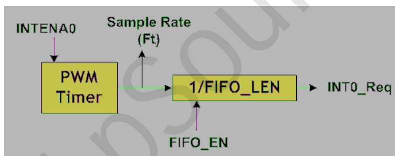
Figure 7.1 Audio PWM Timer Structure
