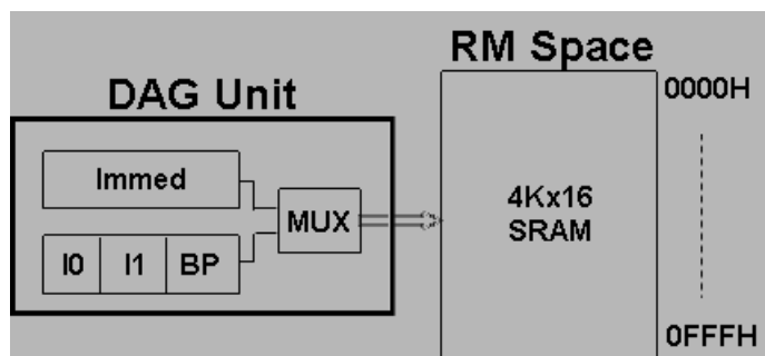
Figure 6.2 RM block diagram
